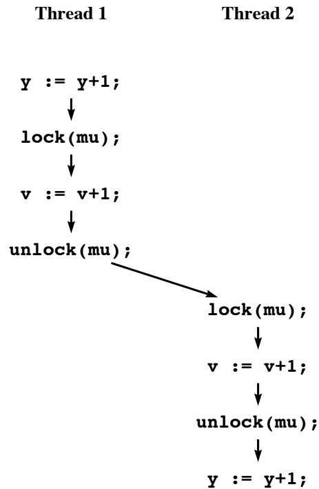
Figure 2: The program allows a data race on y , but the error is not detected by happens-before in this execution interleaving.
